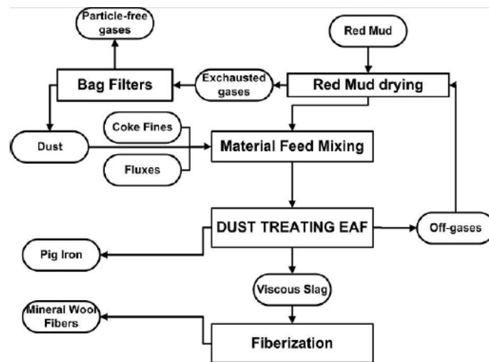
Figure 3: ENEXAL BR treatment flowsheet 2
