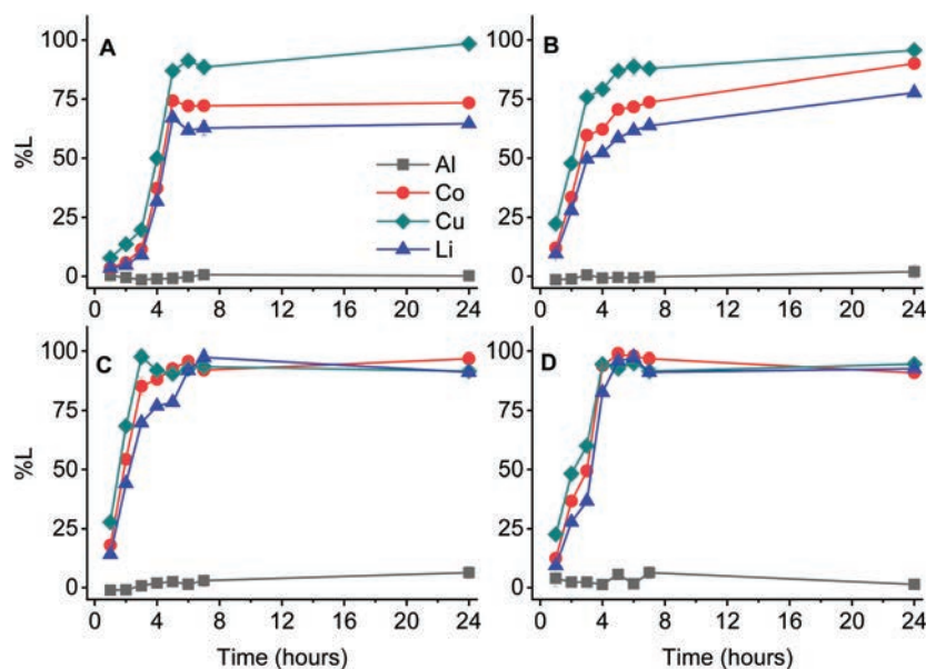
Fig. 4 The percentage leaching during time by 75 vol% (diluted in an aliphatic diluent) D2EHPA at 40 °C (A), 60 °C (B), 80 °C (C) and 100 °C (D). Leaching parameters: 25 g L -1 , 600 rpm. Al : LiCoO 2 = 12 wt%, Cu : LiCoO 2 = 24 wt%.
