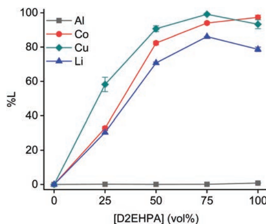
Fig. 2 Percentage leaching by different concentrations of D2EHPA diluted in an aliphatic diluent. Leaching parameters: 80 °C, 8 hours, S:L = 20 g L -1 , 600 rpm. Al:LiCoO 2 = 12 wt%, Cu:LiCoO 2 = 24 wt%.
