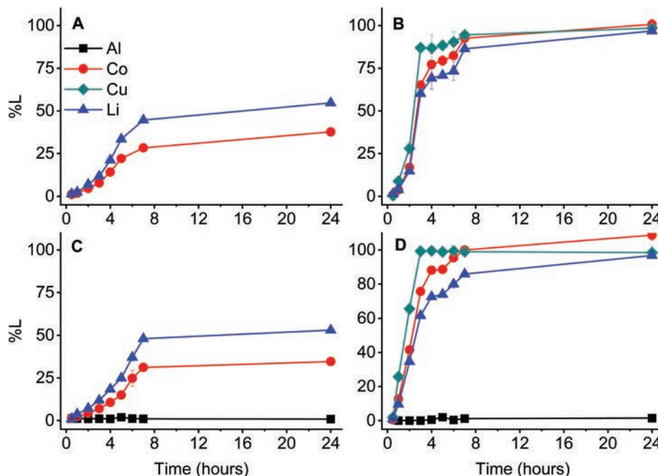
Fig. 5 Leaching efficiencies by 75 vol% (diluted in an aliphatic diluent) D2EHPA during time in four different situations: \text{LiCoO}_2 in absence of Al and Cu (A, left above), \text{LiCoO}_2 in presence of Cu (B, right above), \text{LiCoO}_2 in presence of Al (C, left below) and \text{LiCoO}_2 in presence of both Al and Cu (D, right below). Leaching parameters: 80 °C, 25 g L -1 , 600 rpm. Al : \text{LiCoO}_2 = 12 wt%, Cu : \text{LiCoO}_2 = 24 wt%.
