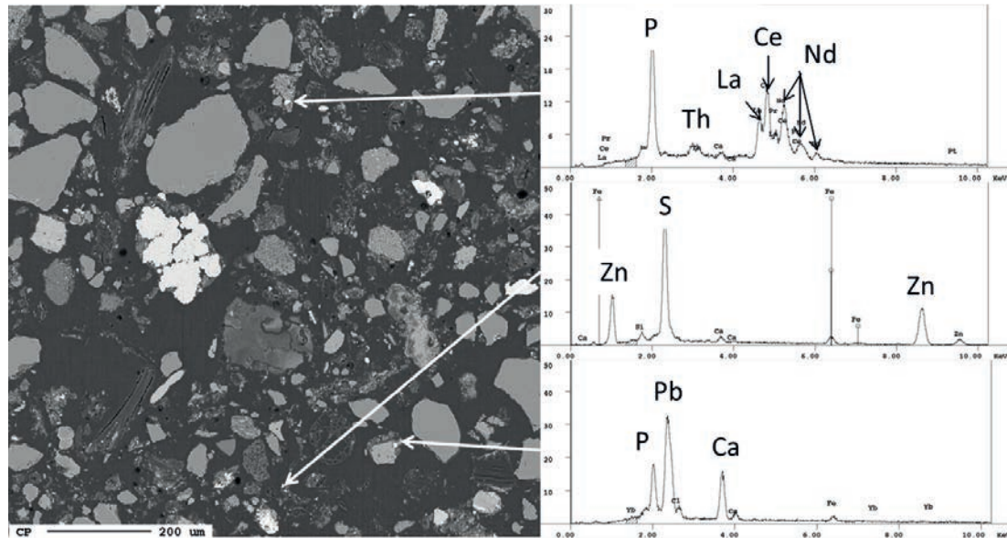
FIGURE 12: Backscattered electron image (left) and EDX spot analyses of heavy metal bearing phases in sample B2_<0.18 mm.
