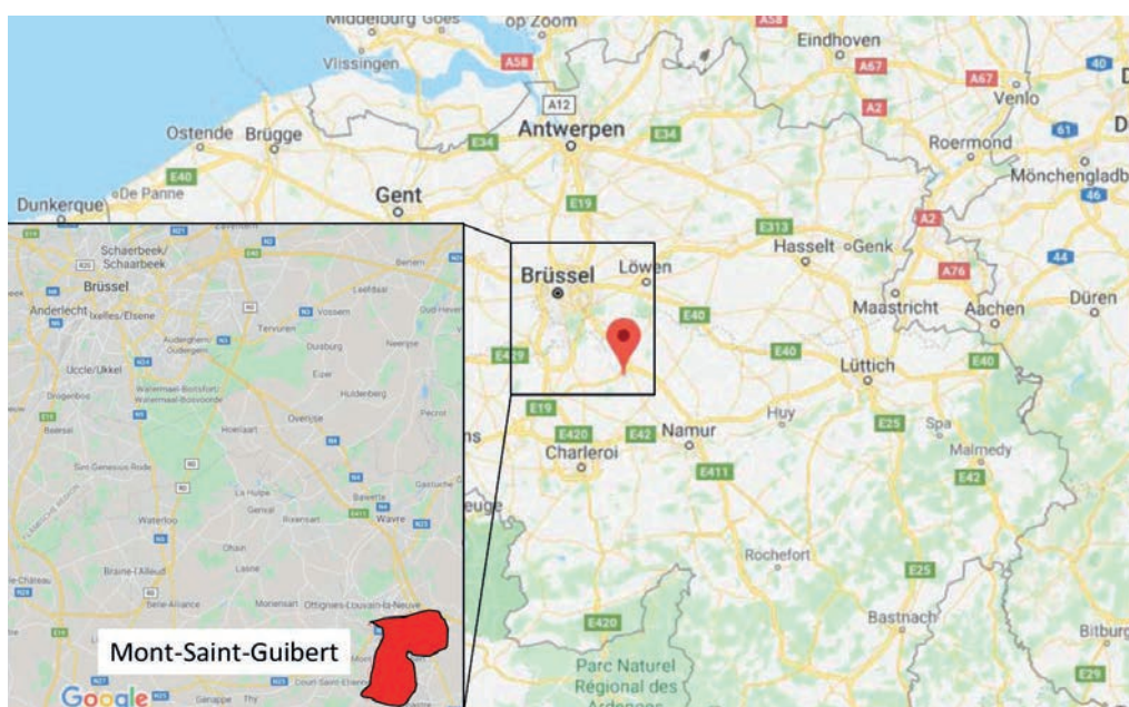
FIGURE 1: Location of the Mont-Saint-Guibert landfill.
