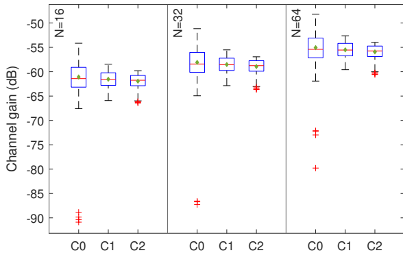
Fig. 6: Channel gain distribution
