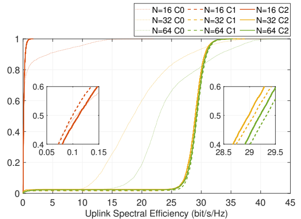
Fig. 7: Capacity performance
