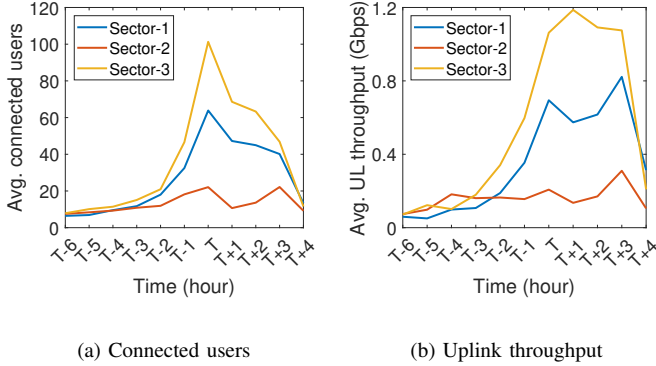
Fig. 1: 5G gNodeB performance in the stadium during match days
